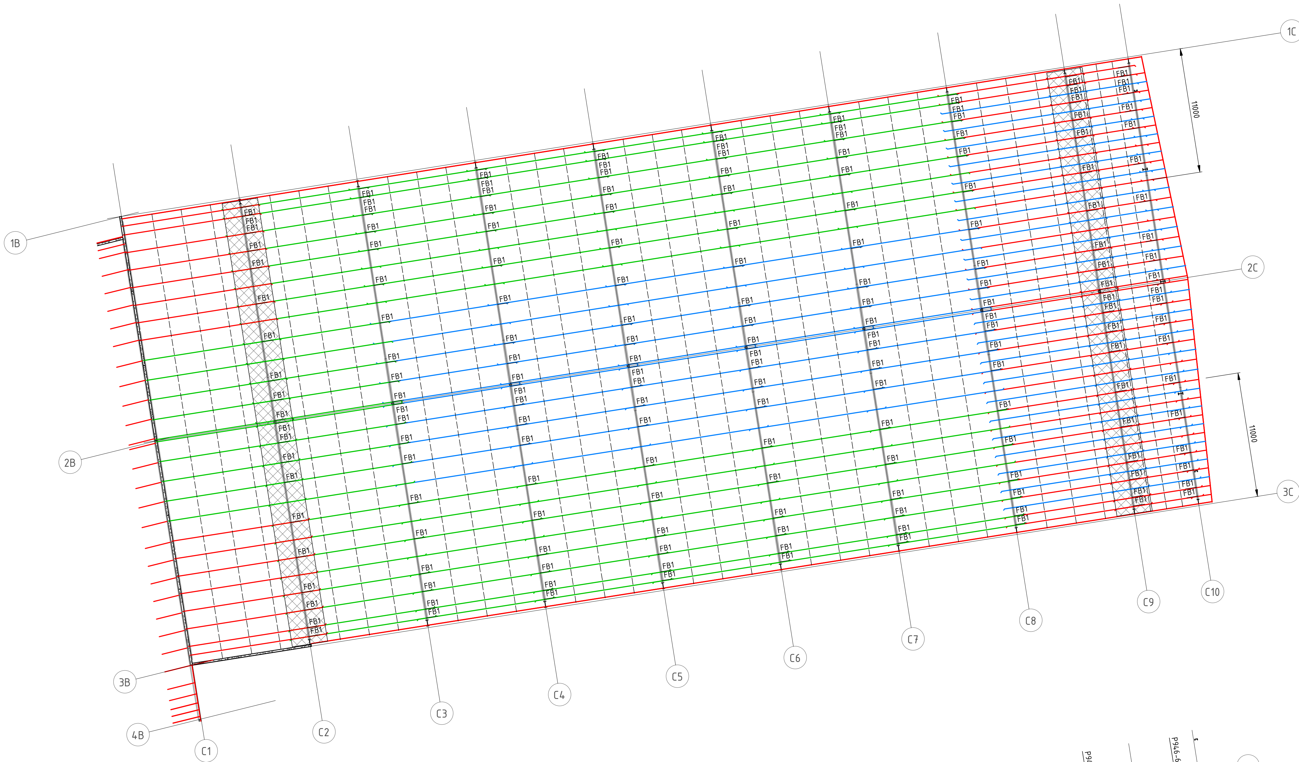
UPPER PURLIN PLAN - PART 3 SCALE 1 : 200
